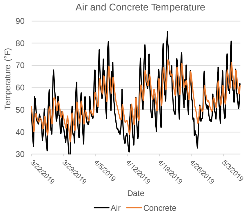
Figure 4.29. Story County 118—air and concrete slab temperatures
