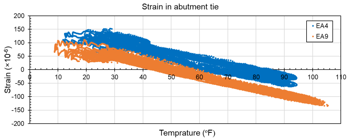
Figure 4.60. Polk County 120—measured strains in the ties, EA4 and EA9
