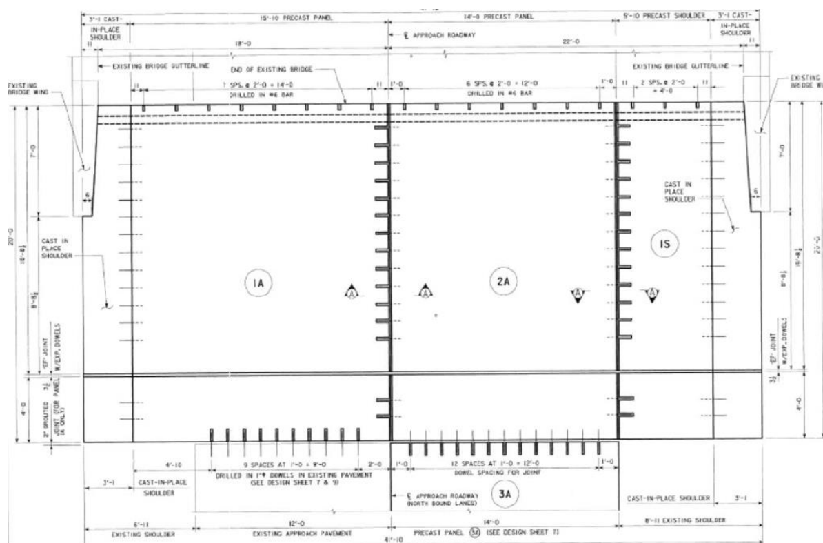
Figure 5.58. Washington County—layout of precast panels at abutment
