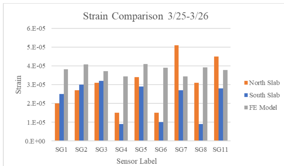
Figure 5.19. Story County 118—approach slab strain comparison
