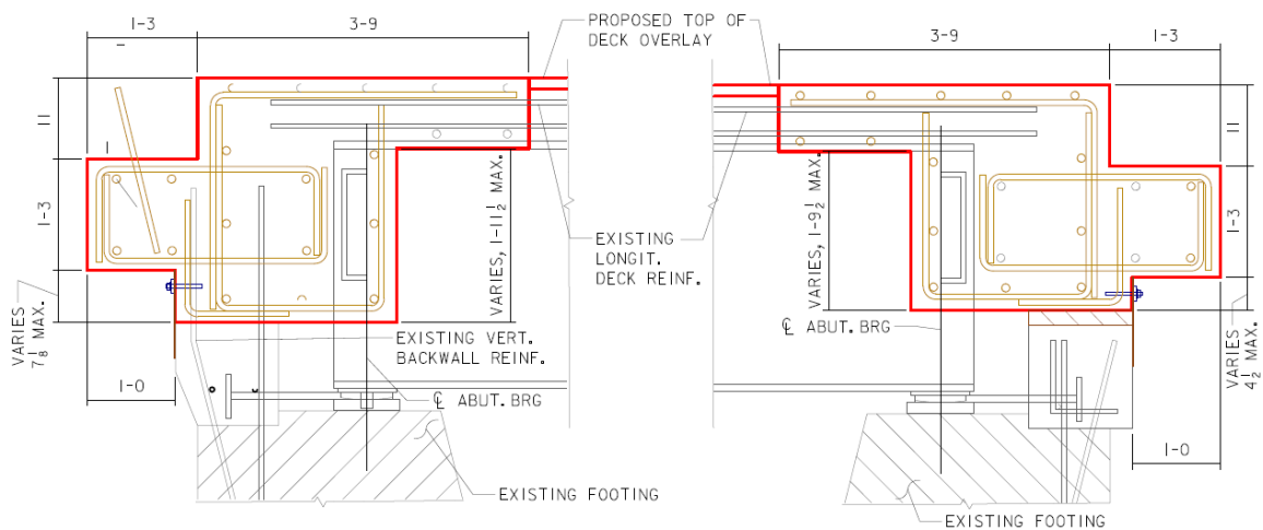
WEST ABUTMENT
