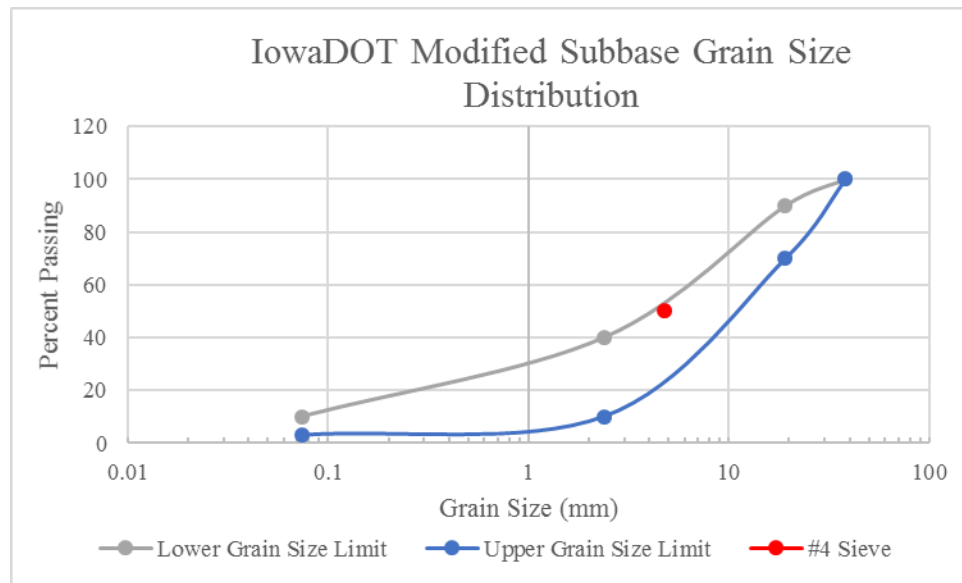
Figure 5.2. Iowa DOT modified subbase grain size distribution
