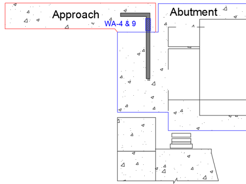
Figure 4.48. Polk County 120—strain gauges in tie
