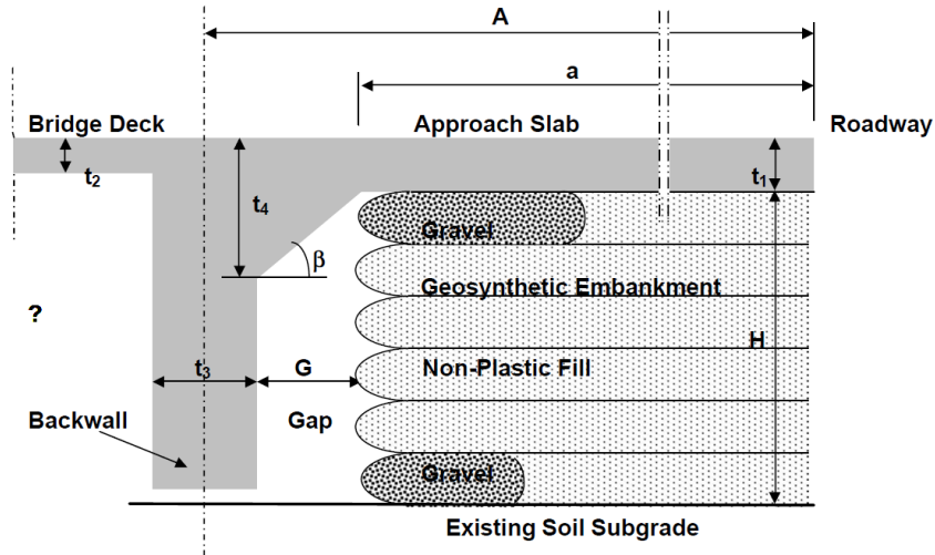
Figure 2.7. Details of Louisiana Department of Transportation and Development (LaDOTD) prototype semi-integral abutment bridge design
