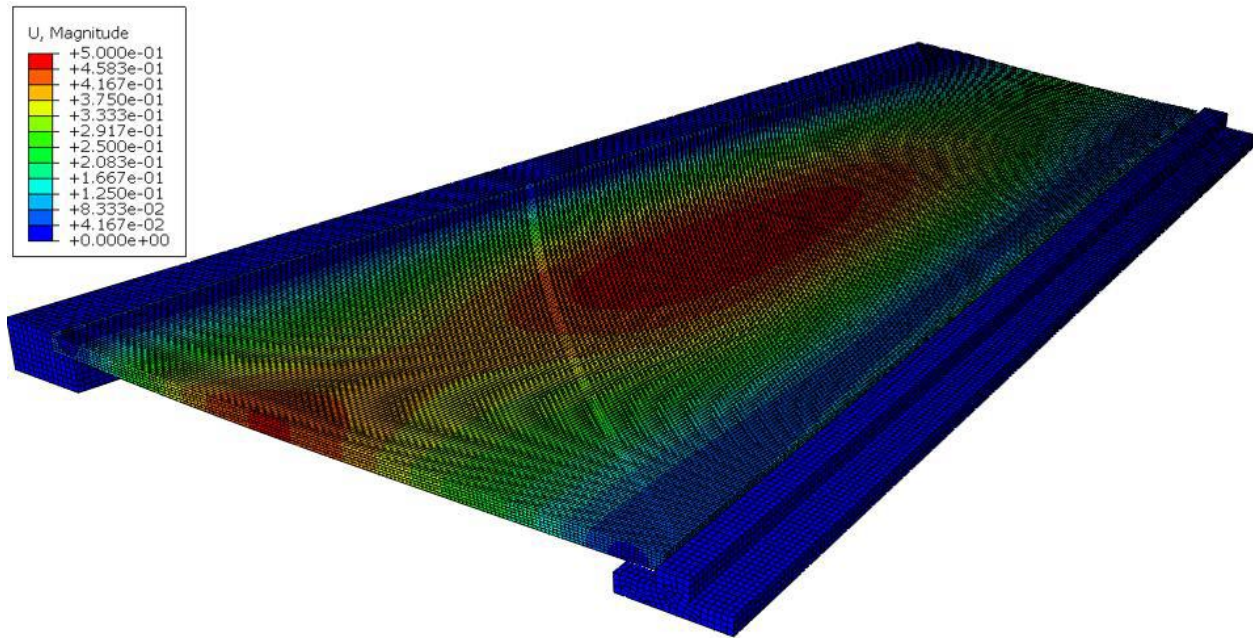
Figure 5.40. Initial vertical settlement for Story County approach slab
