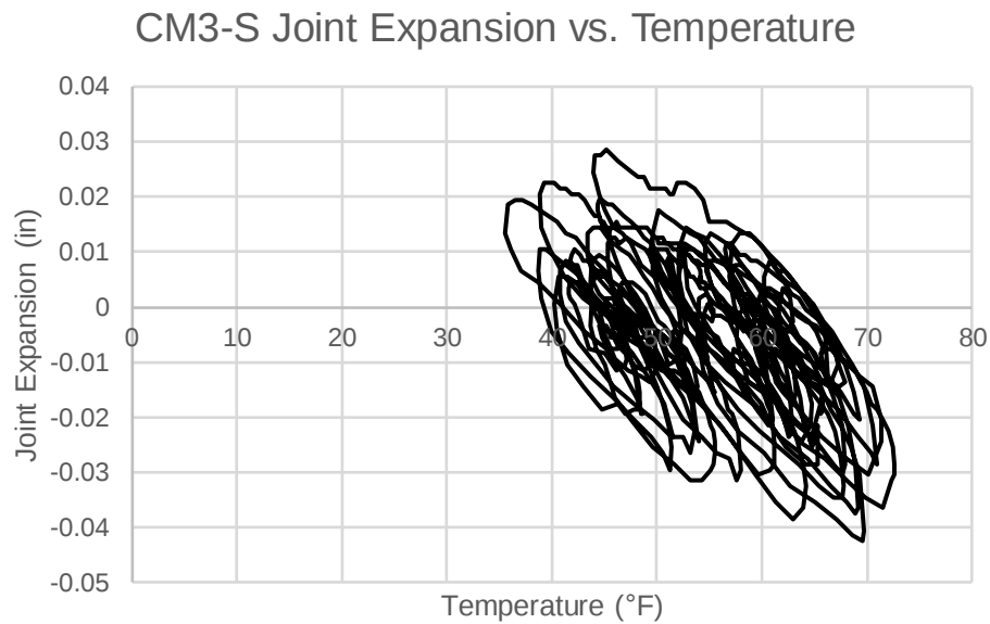
Figure 4.37. Story County 118—bridge-barrier-to-approach-slab-barrier joint expansion
