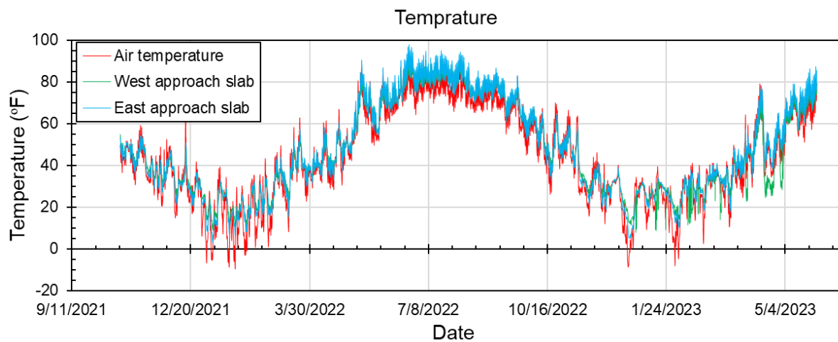
Figure 4.66. Butler County 118—air and concrete slab temperatures
