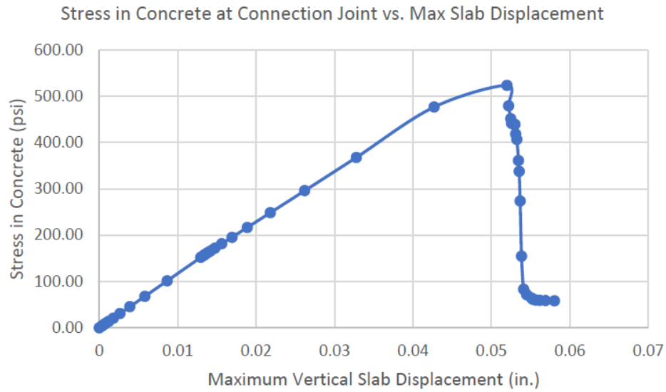
Figure 5.66. Concrete failure in Washington County connection joint
