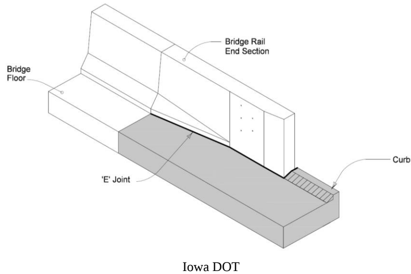
Figure 3.6. Iowa DOT curb E joint detail
