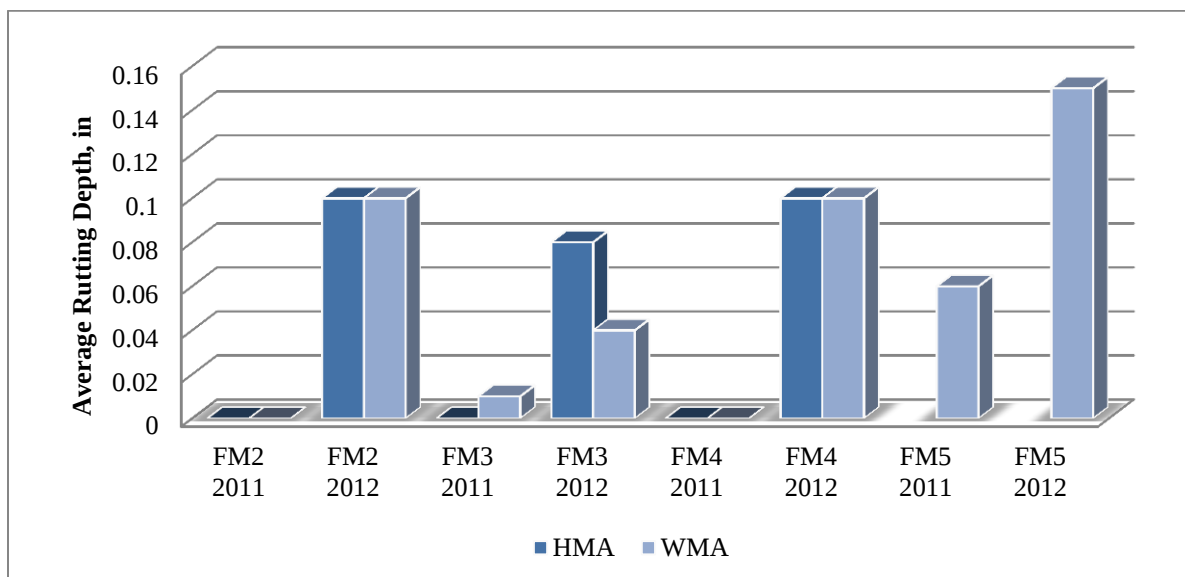
Figure 6.2 Average rutting depth for 2011 and 2012 condition surveys
