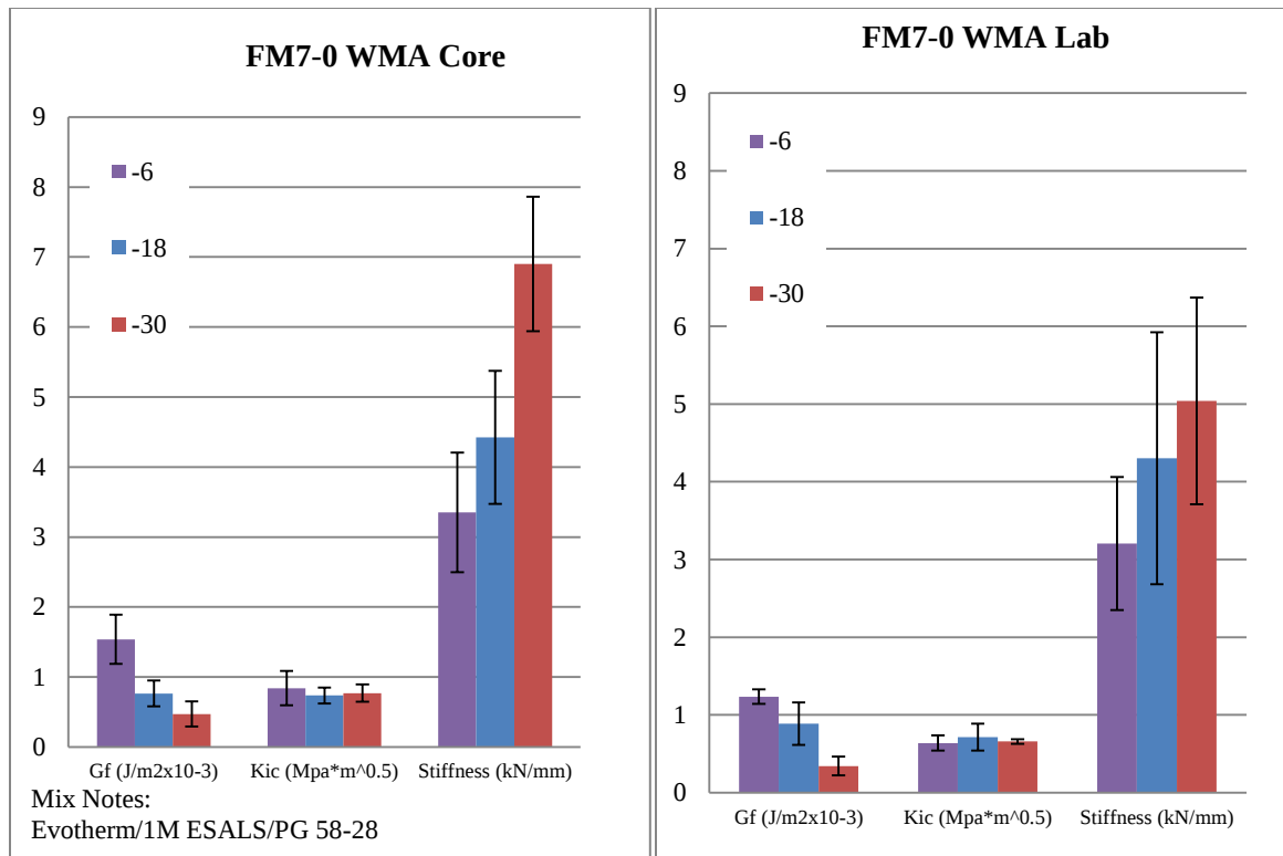
Figure 4.24 SCB results for FM7-0 (Evotherm with 0% Shingles) (Average core air voids are FM7-0=8.4%, FM7-5=7.8 and FM7-7=7.6%; pavement cored after 1 year of service life)
