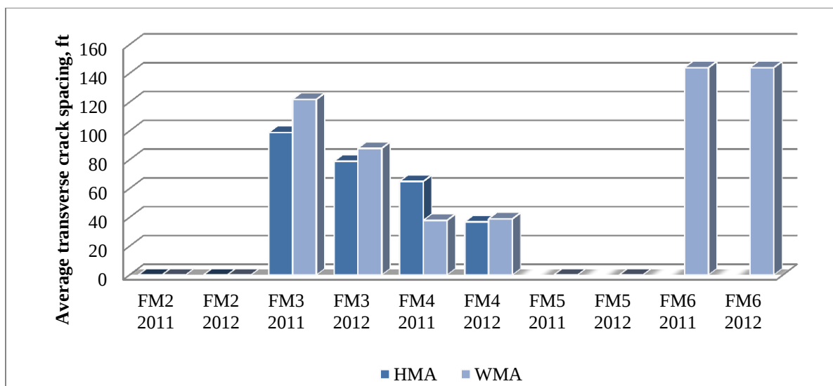
Figure 6.1 Average transverse crack spacing for 2011 and 2012 condition surveys
