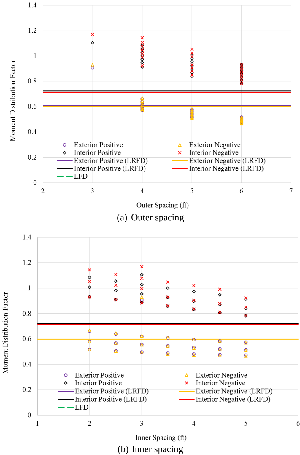
Figure 3.8 Comparisons of moment LDFs with LRFD and LFD results
