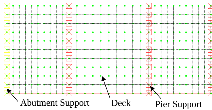
(b) Typical FE model of slab bridge
