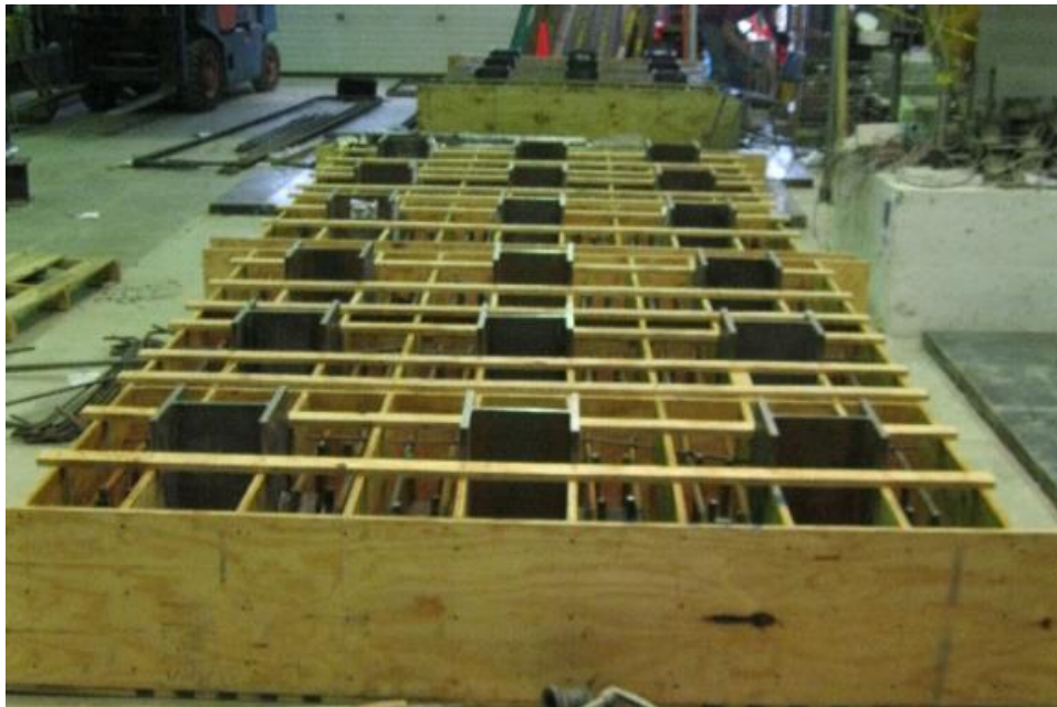
Figure 42. Partially removed concrete specimens and formwork (Dang 2013)
