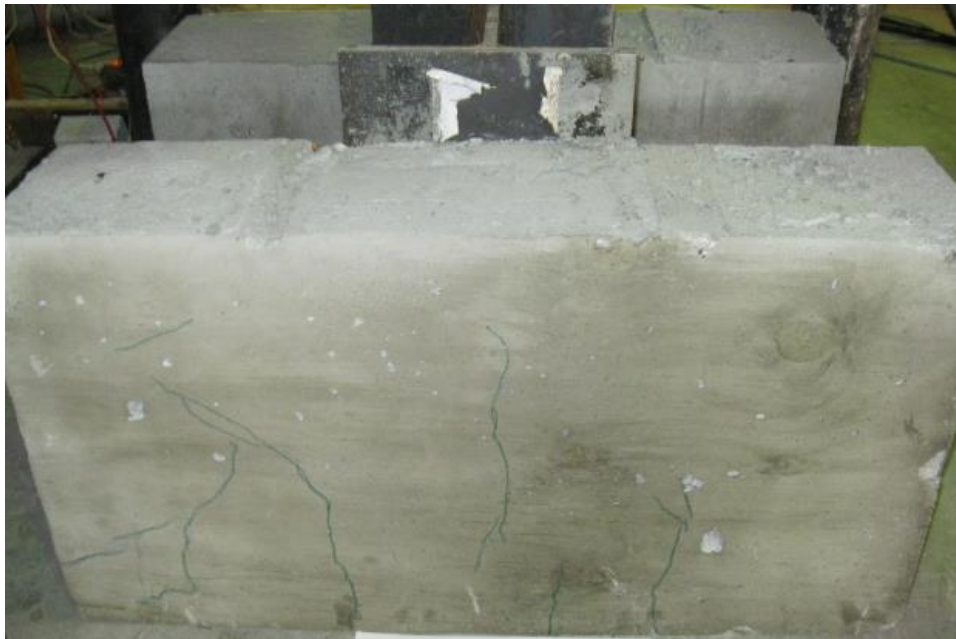
Figure 46. Typical concrete failure (Dang 2013)
