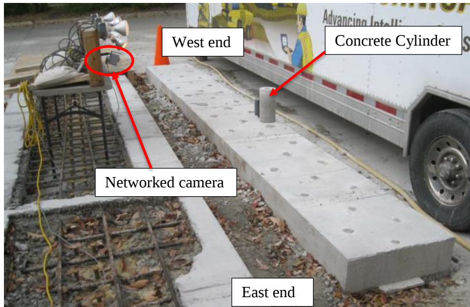
Figure 16. Networked camera and the chemical splitting specimen (Dang 2013)
