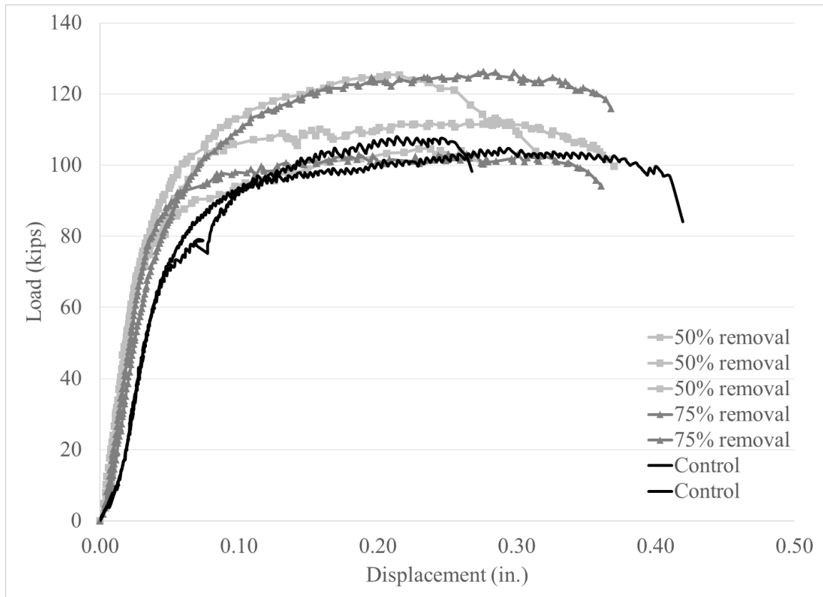
Figure 47. Load verses the average displacement for stud shear connectors
