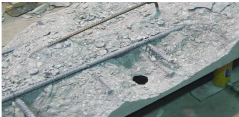
Figure 31. Fourth peeling test (3 shear studs) (Dang 2013)
