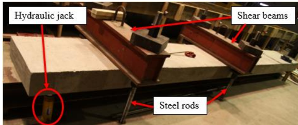
Figure 26. Peeling trial setup
