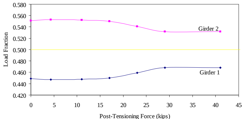
Figure 4.5. Load fractions at midspan for various post-tensioning forces and load at B1
