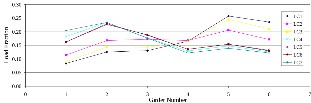
a. 2007 midspan load fraction for seven load cases
