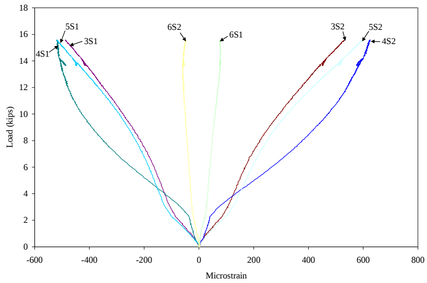
Figure 4.26. Post strains during test 2
