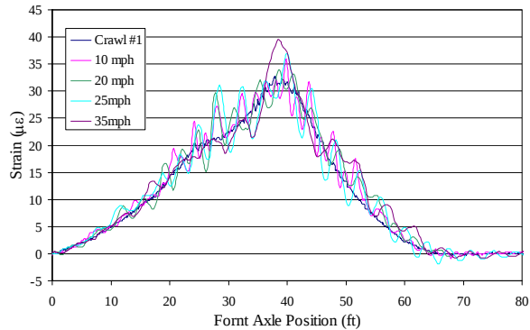
b. 2008 response LC4
