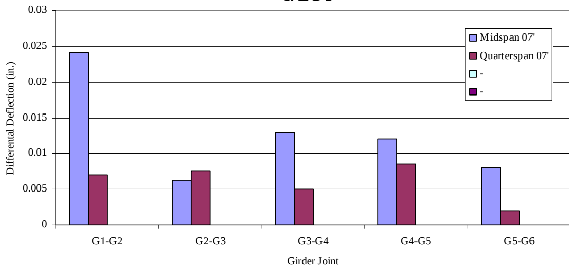
Figure 6.3. 2007 and 2008 differential deflections
