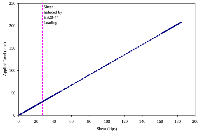
Figure 4.14. Shear force in the box girder
