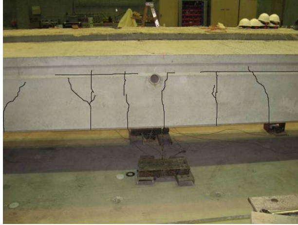
Figure 4.7. Photograph of flexural cracking after flexure test
