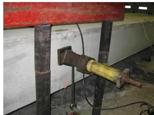
d. post-tensioning bar and jack
