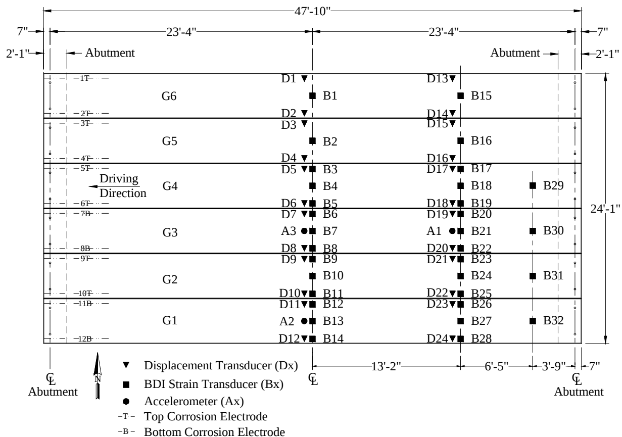
Figure 5.1. Instrumentation layout
