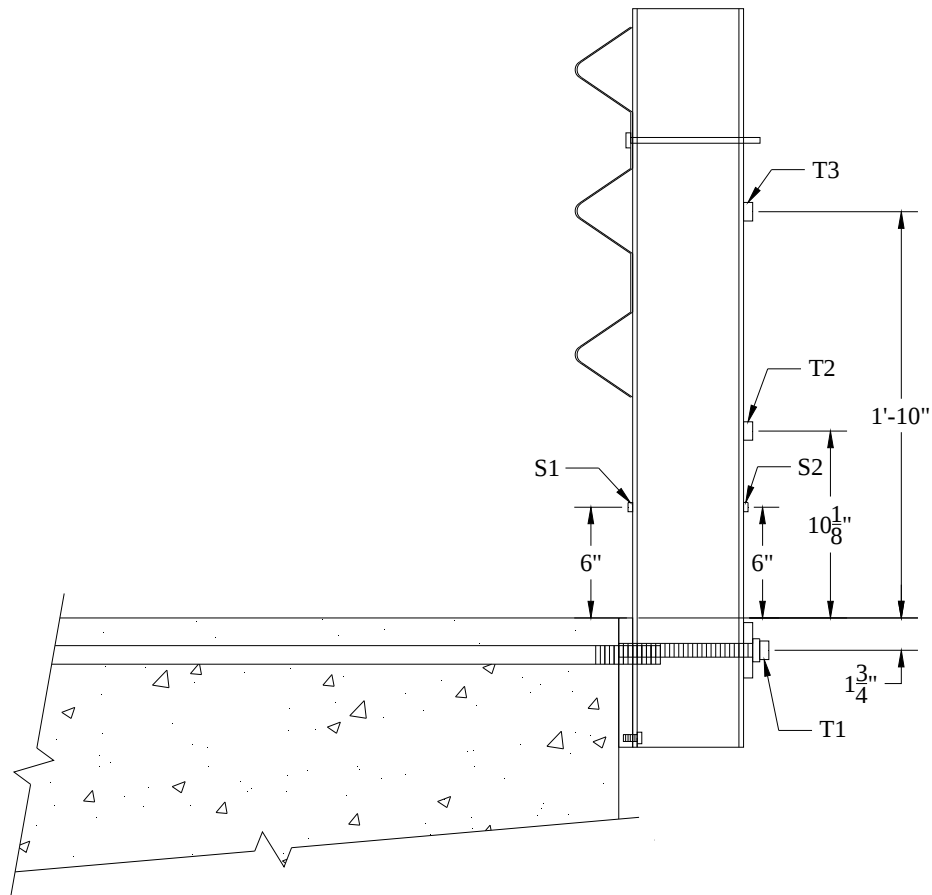
b. guardrail post instrumentation locations
