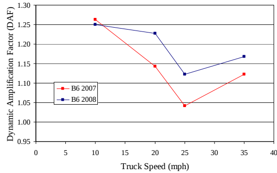
Figure 6.12. 2007 and 2008 DAF LC 2
