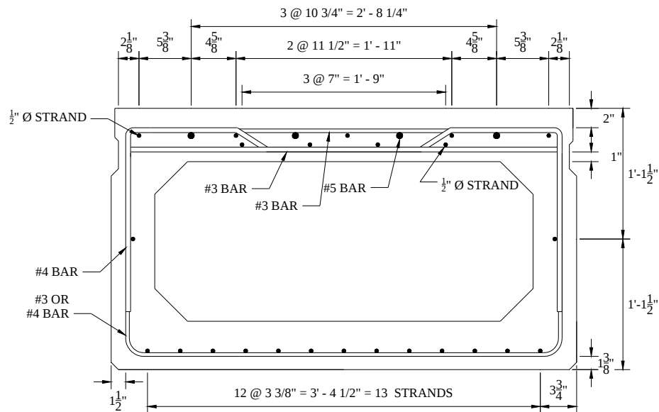
c. section A-A
