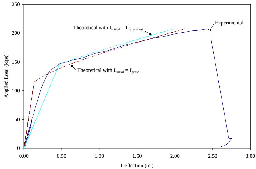
Figure 4.17. Theoretical and experimental deflections at quarterspan during shear test
