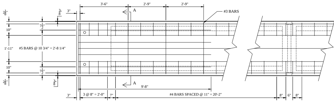
a. top of top slab reinforcement
