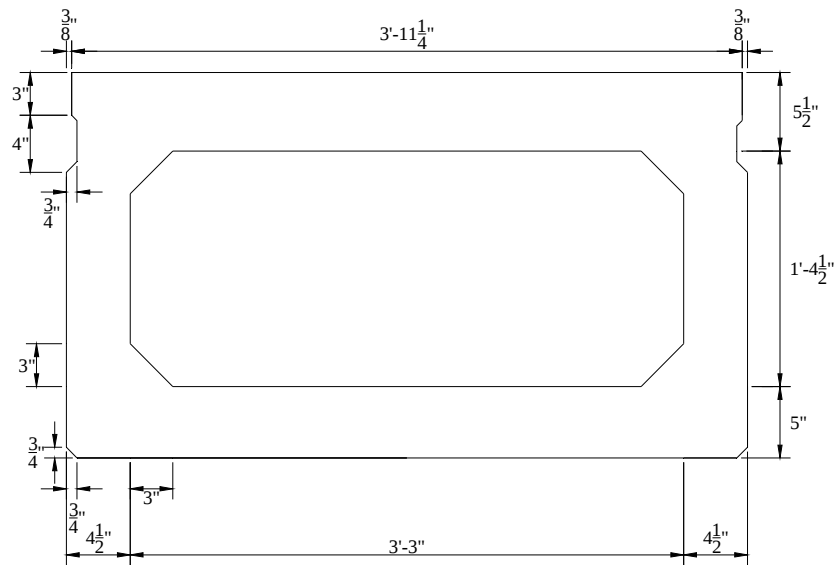
c. section A-A
