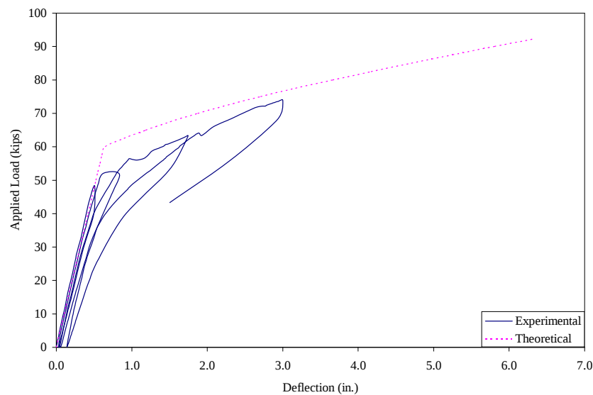
Figure 4.12. Deflection versus load plot for box girder flexural strength test
