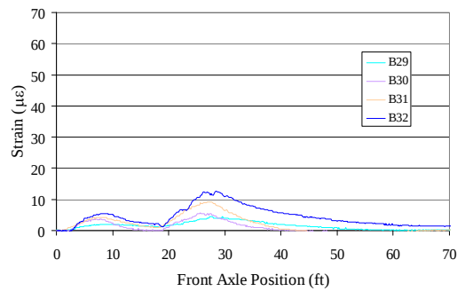
c. eighthspan strain
