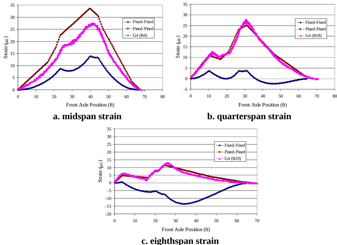
Figure 6.6. 2007 Experimental and analytical strain comparison; LC 3
