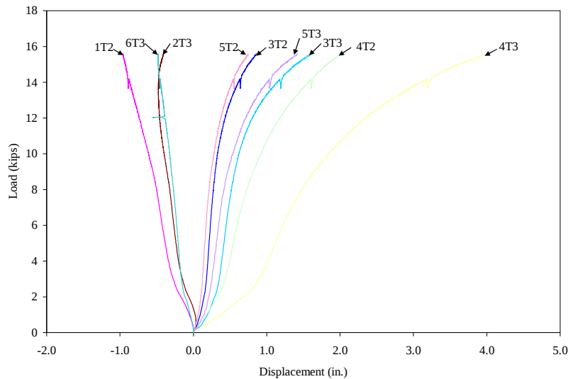
Figure 4.23. Post displacements for test 2
