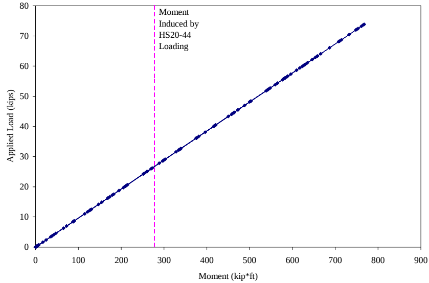
Figure 4.8. Moment at midspan of the box girder
