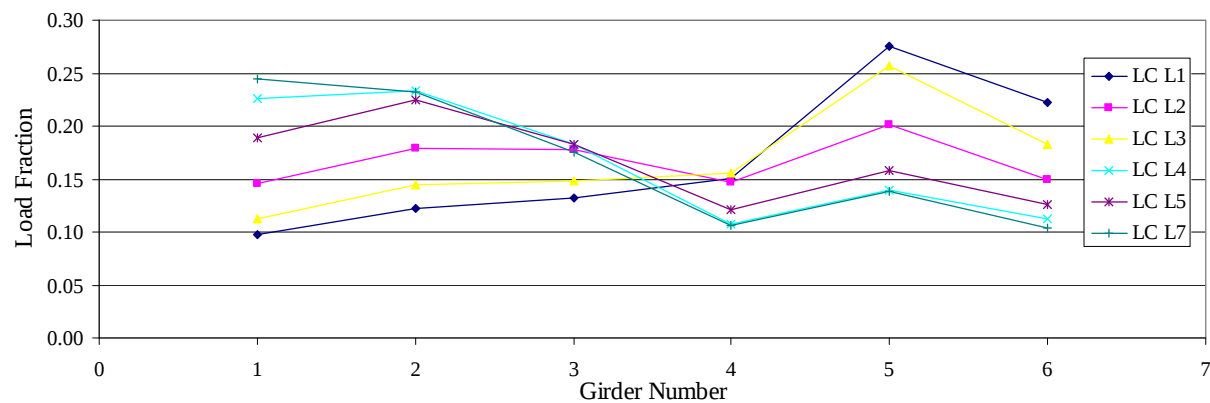
b. 2008 midspan load fraction for six load cases
