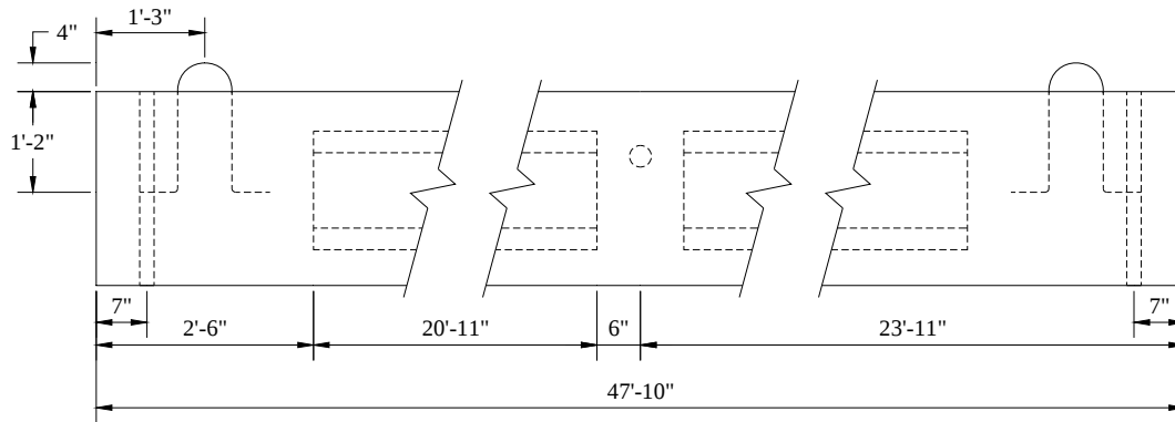
a. profile view
