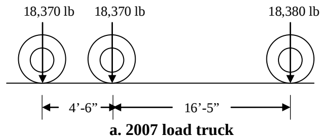
Figure 5.3. Madison County load truck
