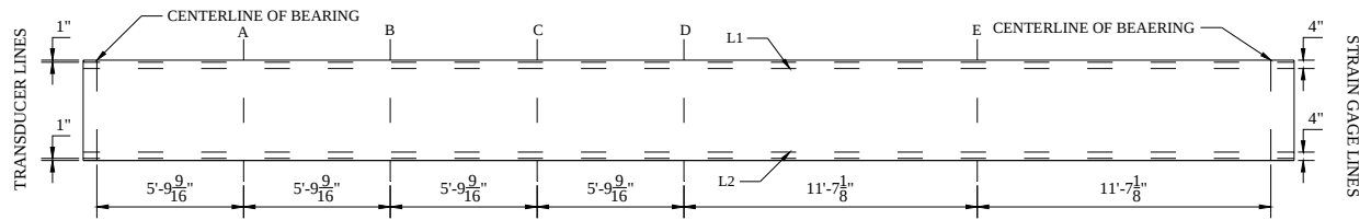
Figure 3.10. Transducer and concrete strain gage grid for shear strength test
