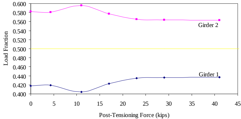
Figure 4.6. Load fractions at quarterspan for various post-tensioning forces and load at B1
