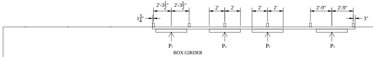
Figure 3.12. Guardrail connection test load locations
