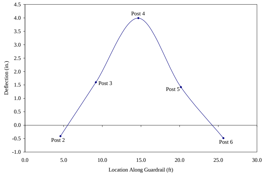
Figure 4.24. Deflected shape of the guardrail during test 2
