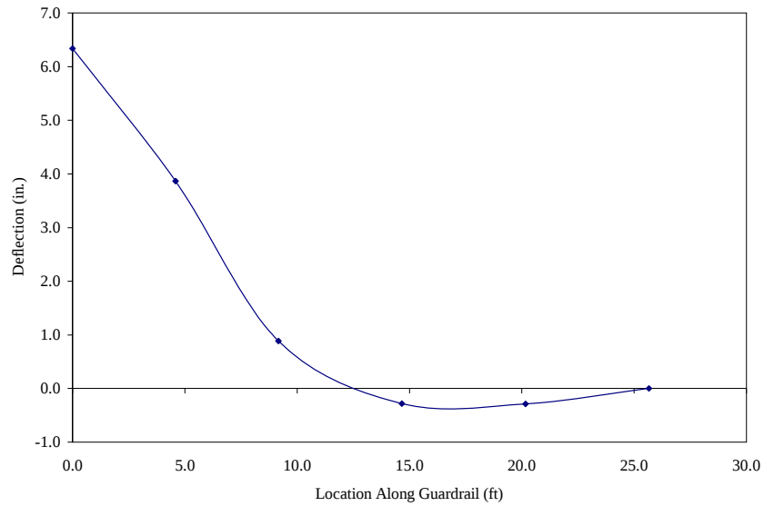
Figure 4.21. Deflected shape of the top of the guardrail at failure
