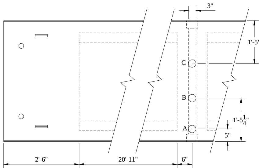
Figure 3.2. Box girder concrete core locations
