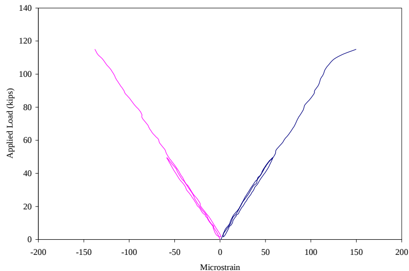
Figure 4.15. Principle strains due to applied load at rosette 2N during shear strength testing
