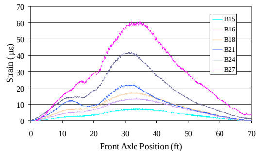
b. quarterspan strain
