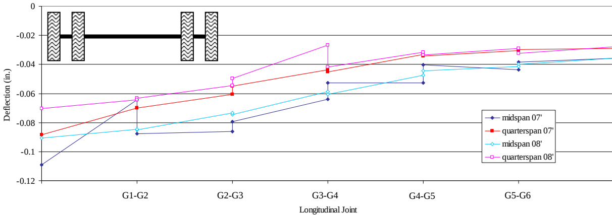
Figure 6.2. 2007 and 2008 transverse deflected shape at midspan and quarterspan
