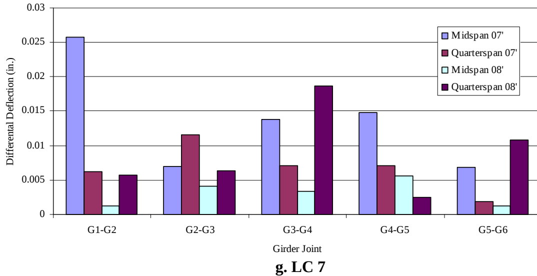
Figure 6.3. 2007 and 2008 differential deflections
