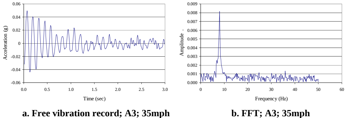
Figure 6.15. Acceleration and frequency plots for 2007 testing
