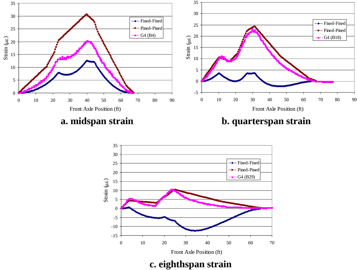
Figure 6.7. 2008 Experimental and analytical strain comparison; LC 3
