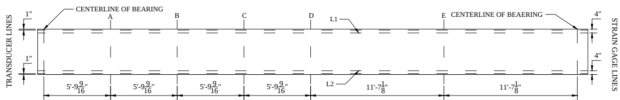
Figure 3.8. Instrumentation locations
