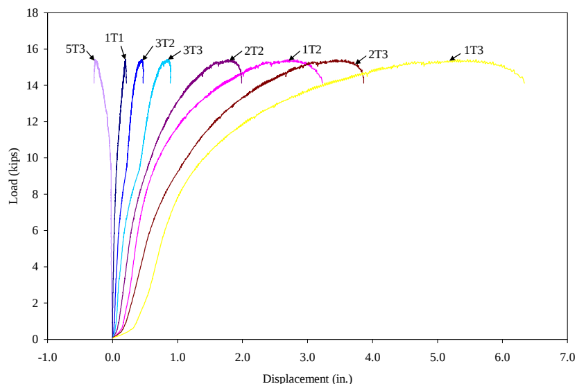
Figure 4.20. Post deflections during test 1
