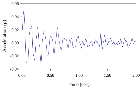
a. Free vibration record; A3; 35mph
