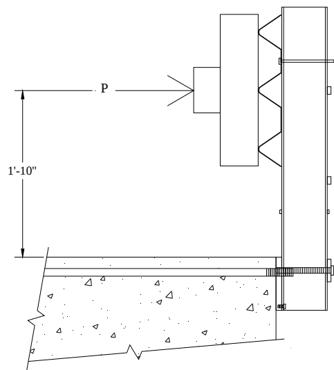
a. profile view of test setup
