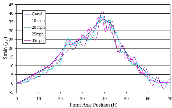
a. 2007 response LC7
