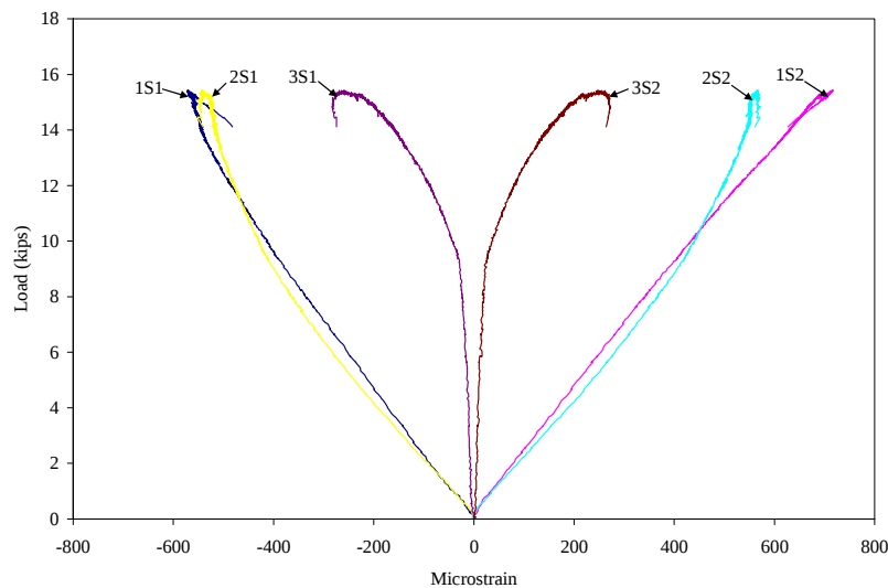
Figure 4.22. Post strains during test 1
