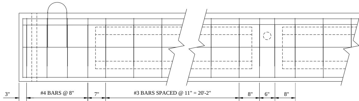
d. profile view of reinforcing layout
