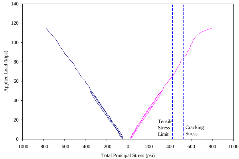
Figure 4.16. Principal stresses due to the total load at rosette 2N
