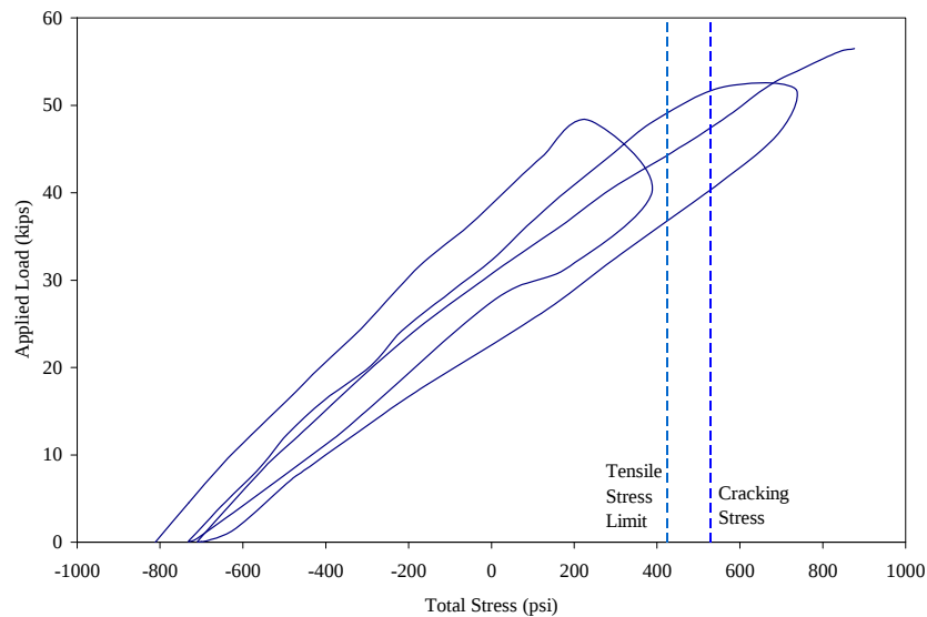
Figure 4.9. Tensile stress at midspan of the box girder
