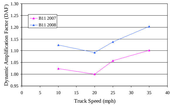
Figure 6.14. 2007 and 2008 DAF LC7
