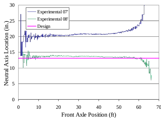
c. Girder G1, LC5
