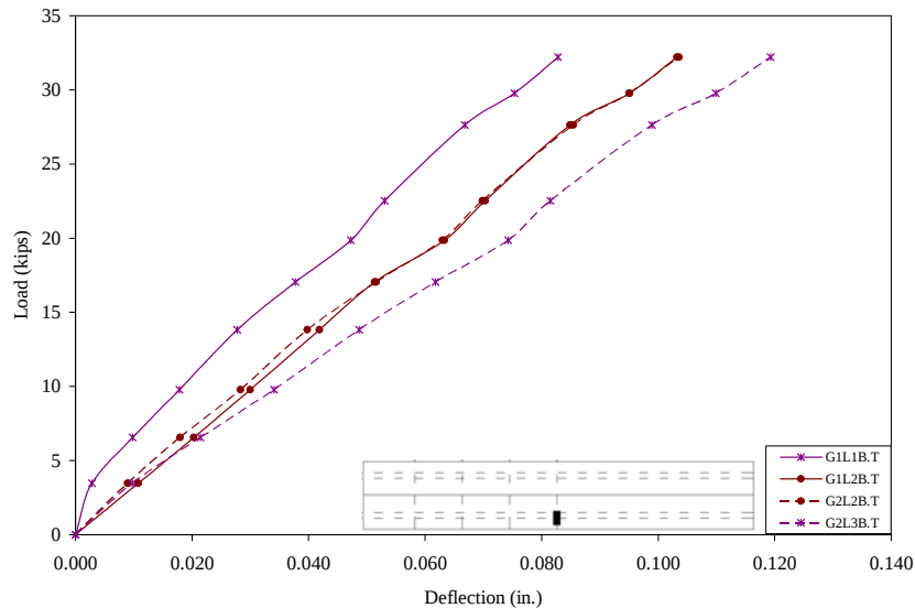
b. deflections at quarterspan
