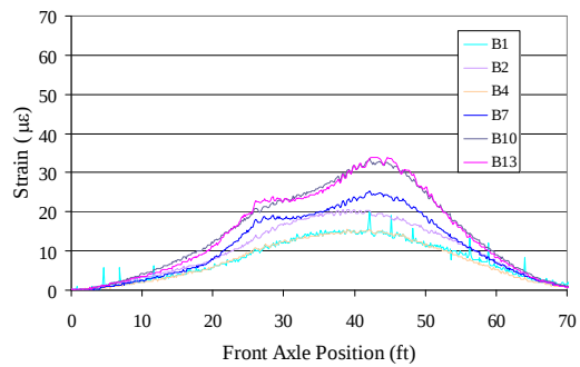
a. midspan strain
