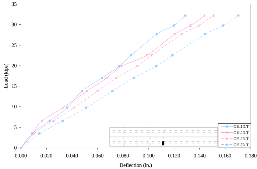
a. deflections at midspan
