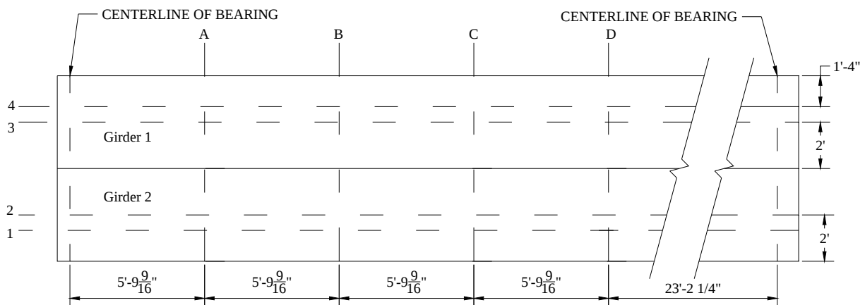
Figure 3.4. Variable post-tensioning loading locations
