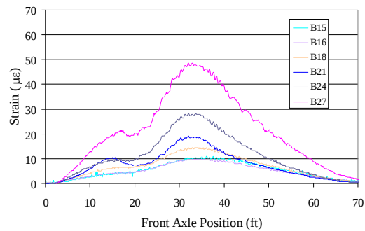
b. quarterspan strain
