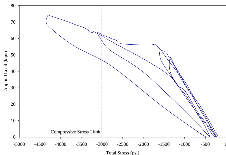
Figure 4.10. Total compressive stress at midspan of the box girder
