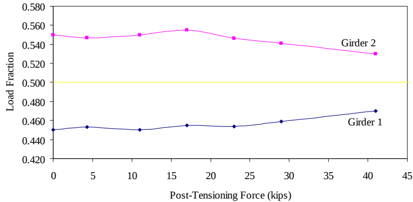
Figure 4.4. Load fractions at quarterspan for various post-tensioning forces and load at D1
