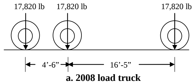
Figure 5.4. Vehicle configuration and axle loads
