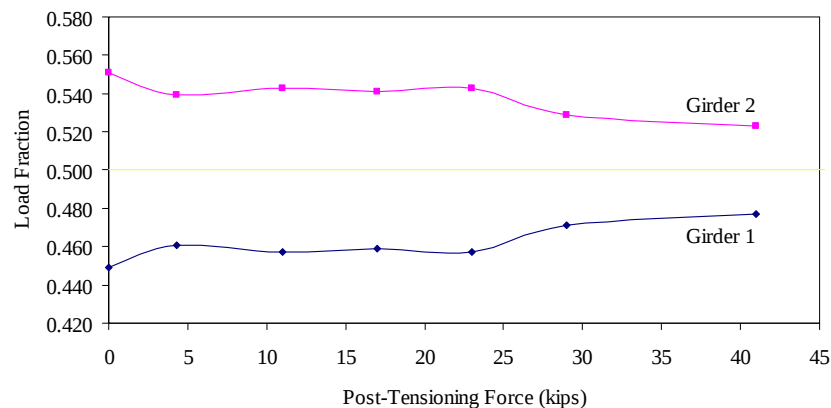
Figure 4.3. Load fractions at midspan for various post-tensioning forces and load at D1
