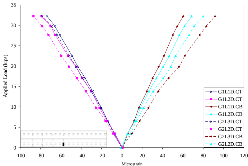
Figure 4.1. Total strain at midspan with load at D1 and a post-tensioning force of 17 kips
