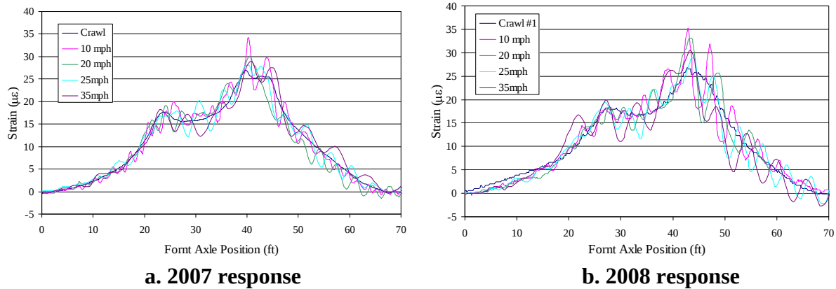
Figure 6.11. Transducer B6 dynamic response LC2
