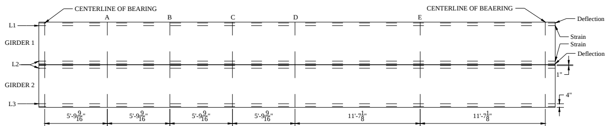
Figure 3.6. Instrumentation grid for variable post-tensioning force tests
