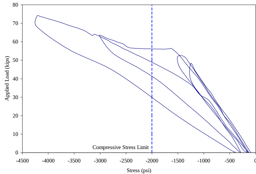
Figure 4.11. Compressive stress due to applied load and one-half the dead load and prestressing force at midspan of the box girder
